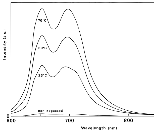
Figure 4. Low-resolution fluorescence spectra of a 1.4 × 10 -6 M solution of C 70 in liquid paraffin. Degassed solution at 23, 50, and 70 °C. The intensity of the nondegassed solution is independent of temperature, and is entirely due to prompt fluorescence. The rise with temperature observed in the degassed solutions results from the increasing contribution of delayed fluorescence to the total intensity. Emission slits were 9 nm.
