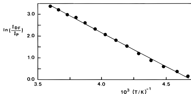
Figure 3. Log plot of the intensity ratio of delayed fluorescence to phosphorescence vs 1/T, from -59 to 5 °C. Emission wavelengths were 688 (delayed fluorescence) and 832 nm (phosphorescence). [C 70 ] = 1.1 × 10 -5 M.
