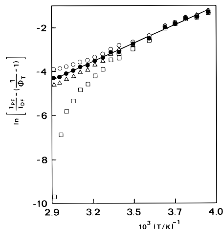
Figure 5. Fit of I_{PF}/I_{DF} vs 1/T, according to eq 6, for temperatures from -20 to 70 °C. The effect of \Phi_T on the linearity is clear: \Phi_T = 1.000 (○), 0.994 (●) (best value), 0.990 (△), and 0.980 (□). Excitation and emission slits were 18 and 9 nm, respectively.
