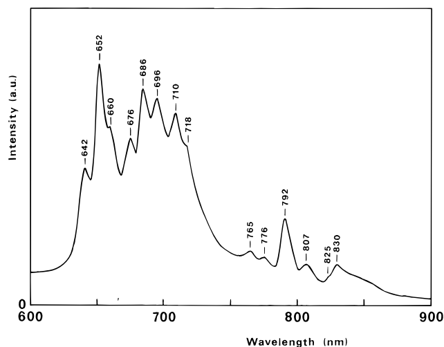
Figure 2. Luminescence spectrum of C 70 dissolved in paraffin, at -30 °C. [C 70 ] = 2.5 × 10 -5 M. Excitation and emission slits were 18 and 2 nm, respectively. The fluorescence spans the range 630–750 nm. The fluorescence band at 642 nm appears to be a hot band. The phosphorescence begins at ca. 750 nm, and extends further to the infrared (not shown). Peak wavelengths have an estimated accuracy of ±1 nm.
